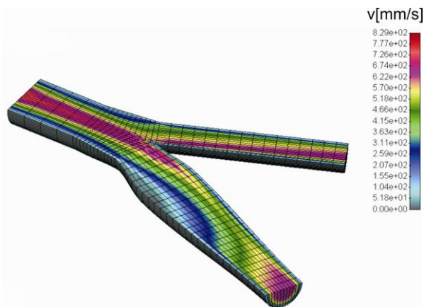
Fig. 9 3D field of velocity magnitude at the maximum systolic flow (at relative time t/T = 0.11 within the period T ).
