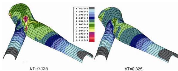
Fig. 10 Distribution of von Mises stress, Pa within the artery walls of the carotid artery bifurcation due to action of blood, for systolic deceleration flow, t/T=0.125 and diastolic minimum flow, t/T=0.325 .
